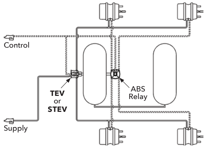
TEV & STEV System
