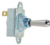
422642 ON/OFF SPST S SCREWS 50 AMPS 12 Volts
