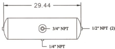
8" dia. Air Tanks 1425 cubic inch capacity (6.16 Gallons)
