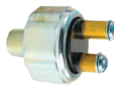
422710 STOP LAMP SWITCH NORMALLY OFF SPST OPERATES 60-120 PSI CONTACT CLOSED AT RISING PRESSURE
